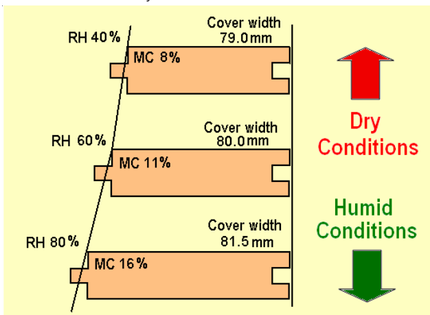
Figure 1 – Cover width variation with changing Relative Humidity
