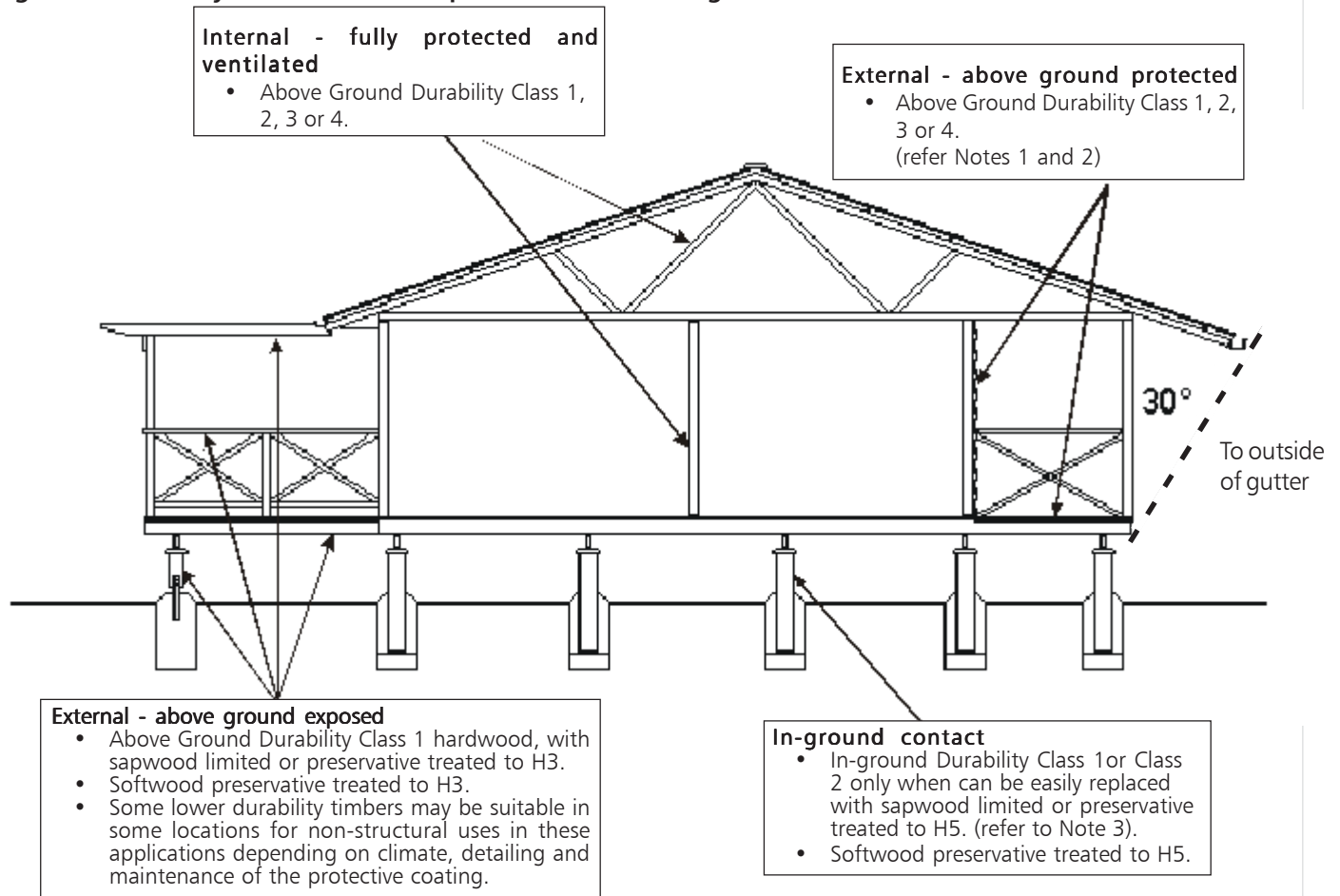
Figure 1: Durability and Treatment Requirements for Housing
